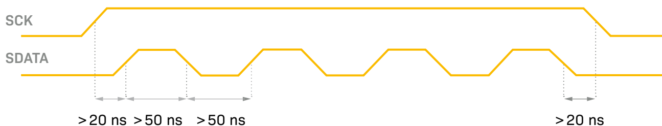
Figure 4.1. Reset sequence
